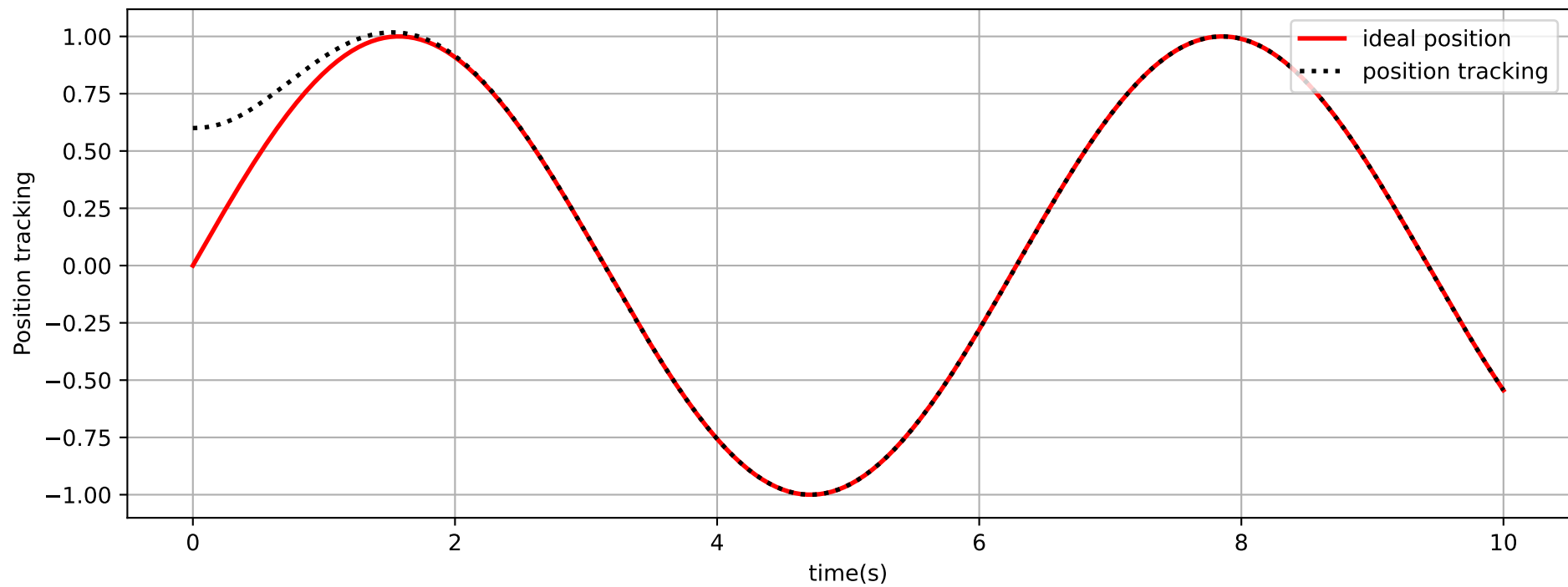
Tracking Performance ( S=2 , S1=1 , m=19 )
